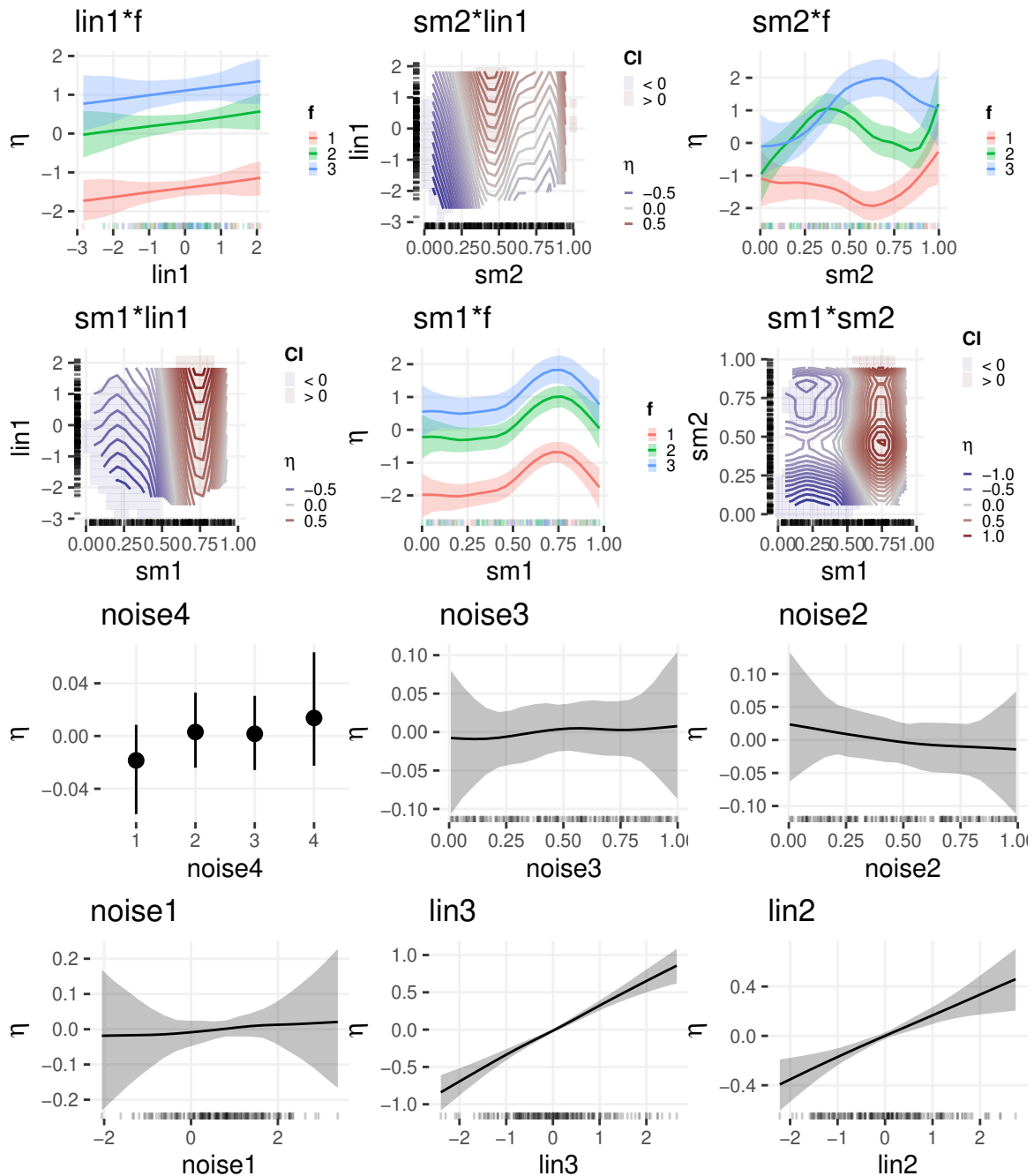
Figure 3: Posterior means and pointwise 80% credible intervals for model m . Interaction surfaces of two numerical covariates are displayed as color coded contour plots, with regions in which the credible interval does not overlap zero marked in blue ( \eta < 0 ) or red ( \eta > 0 ). Each panel contains a marginal rug plot that shows where the observations are located. Note that the default behavior of plot.spikeSlabCAM is to cumulate all terms associated with a covariate or covariate combination. In this example, the joint effects of the first 4 covariates sm1 , sm2 , f and lin1 and the sums of the lin - and sm -terms associated with lin2 , lin3 , noise1 , noise2 and noise3 are displayed. All effects of the noise variables are \approx 0 , note the different scales on the vertical axes. Vertical axes can be forced to the same range by setting option commonEtaScale .
