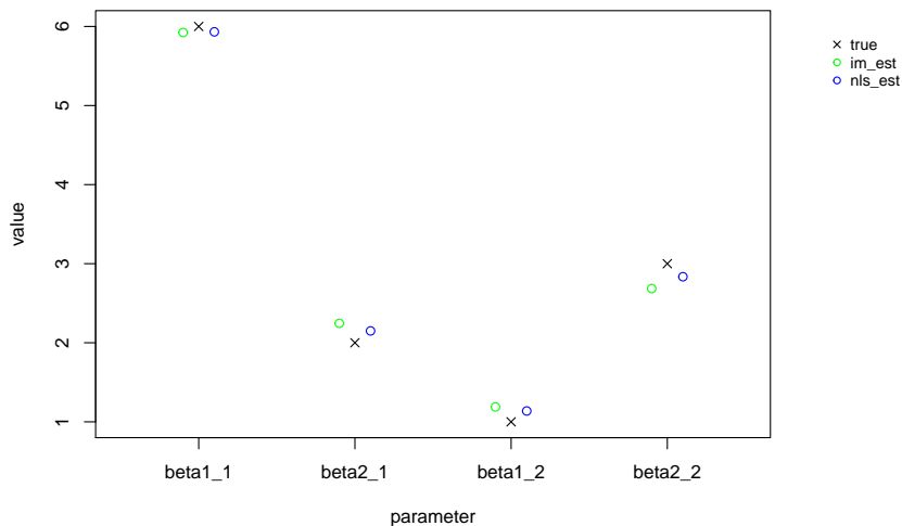
Figure 8: SIR case (a) - estimates of \beta
