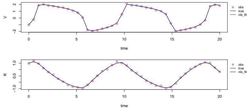
Figure 9: Solutions V and R of the FitzHugh-Nagum model (15), noisy observations and model fits.
