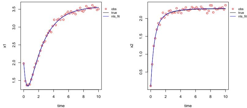
Figure 3: Case (a): 'True' and estimated solutions x_1 and x_2 of the biochemical system of equation (1).
